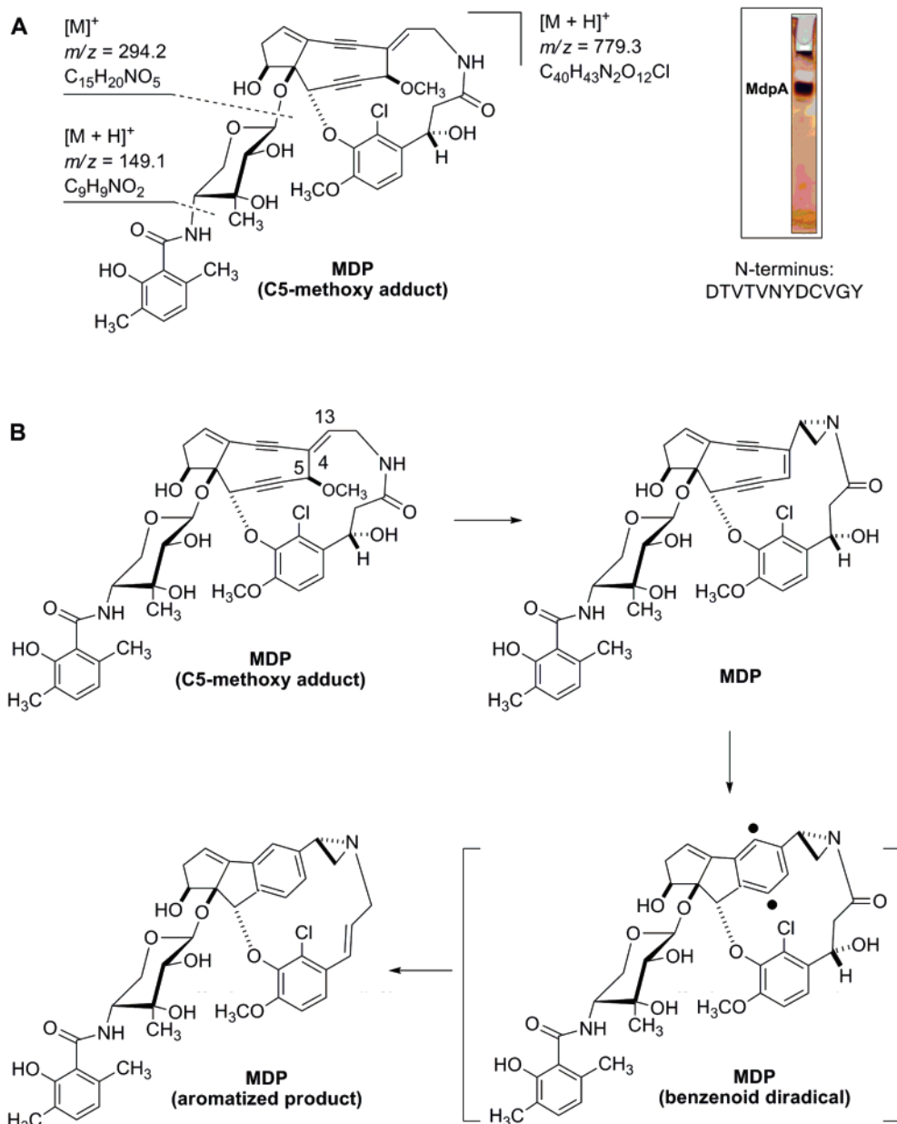
Figure 2. Isolation of MDP chromophore and binding protein, MdpA. (A) The chromophore was purified and confirmed by MS giving the characteristic MDP–OCH 3 adduct and associated mass fragments as reported previously; 14 the MDP binding protein was purified and confirmed by N-terminal sequencing. (B) Isolation of MDP as a MDP–OCH 3 adduct, its rearrangement to the aziridine form MDP, subsequent Bergman rearrangement to afford the MDP–benzenoid diradical, and final formation of the MDP–aromatized product after addition of two hydrogen atoms as described previously. 14
