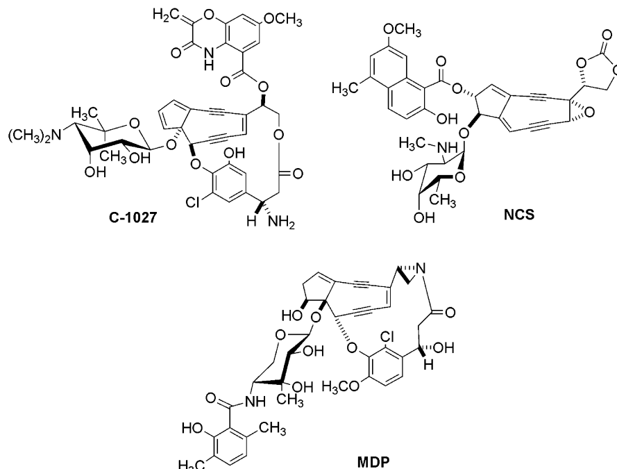
Figure 1. Structures of the nine-membered enediynes C-1027, NCS, and MDP.
