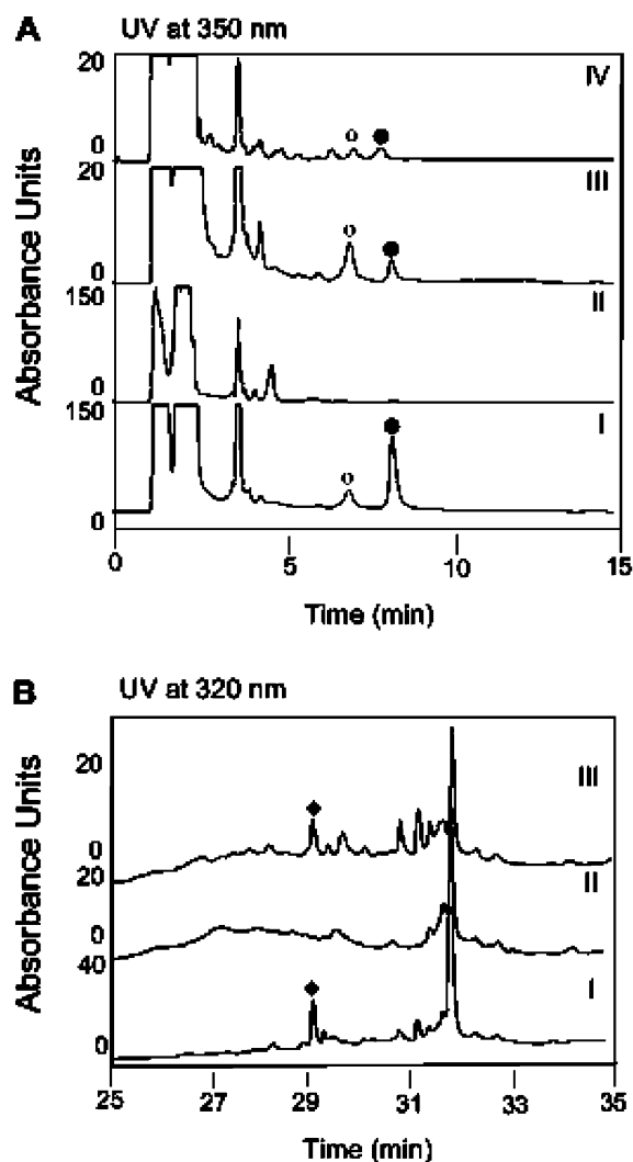
Figure 7. Heterologous complementation of C-1027 and NCS enediyne PKS mutants by the MdpE enediyne PKS cassette. (A) Complementation of C-1027 enediyne polyketide synthase mutant (SB1005) with empty vector (II); sgcE , plasmid pBS1019 (III); and mdpE/E5/E6/E10 , plasmid pBS3010 (IV). For comparisons, production of C-1027 from wild-type producer is shown (I). (B) Complementation of NCS enediyne polyketide synthase mutant (SB5002) with ncsE , plasmid pBS5019 (I); empty vector (II); and mdpE/E5/E6/E10 , plasmid pBS10005 (III). Symbols are (●) for C-1027 in the enediyne form, (○) for C-1027 aromatized product, and (◆) for NCS.
