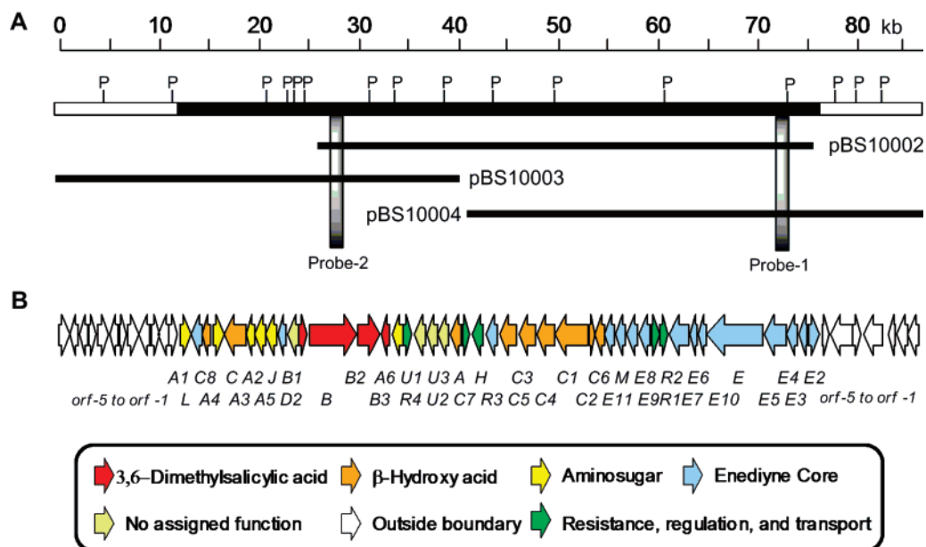
Figure 3. MDP biosynthetic gene cluster from A. madurae ATCC 39144. (A) Restriction map of the 85-kb DNA region encompassed by three overlapping cosmids represented by pBS10002, pBS10003, and pBS10004. Solid black indicates the region whose gene products are predicted to be involved in MDP biosynthesis (62.8 kb). P, Pst I. Probe-1 and -2 were used to localize the overlapping cosmids covering the MDP cluster. (B) Genetic organization of the MDP biosynthetic gene cluster. Proposed functions for individual orfs are color-coded and summarized in Table 1.
